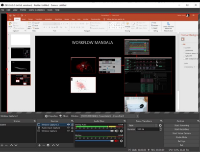
OBS Studio
