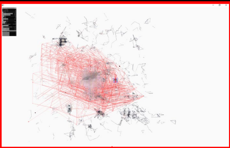
p5.js Sketches
