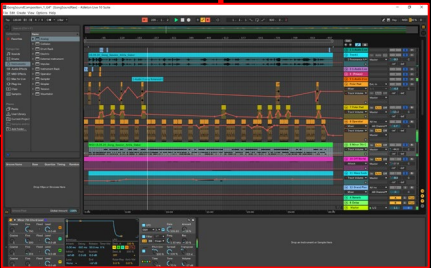
Ableton Live
