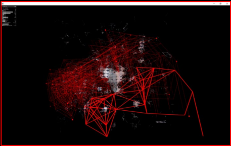
C++ Sketches
